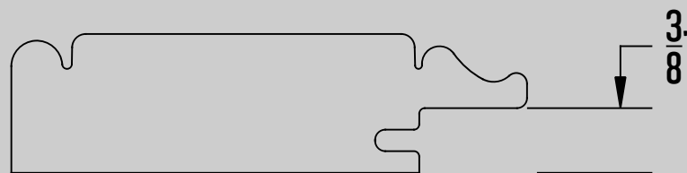
Miter 33 [76mm] RFG
